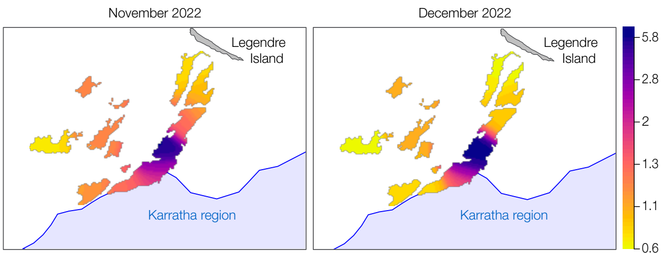
Figure 2: Spatial trends of the NO 2 (mg/m 3 ) gas measurements (IVL passive sampler) from the air quality monitoring sites for November and December 2022
