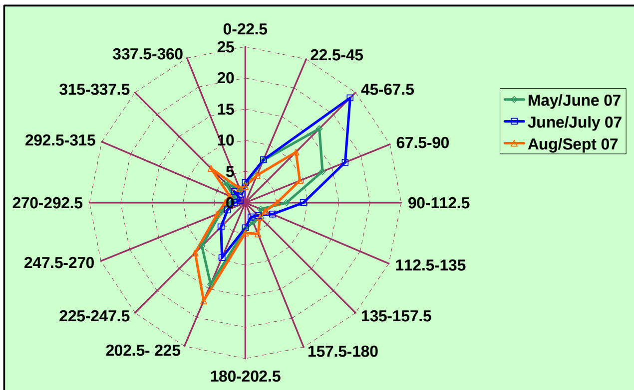
Figure J6. Wind roses recorded at site 8 for three periods from 3 rd May 2007– 7 th June 2007, 7 th June 2007– 3 rd August 2007 and 3 rd August 2007 – 12 th September 2007.
