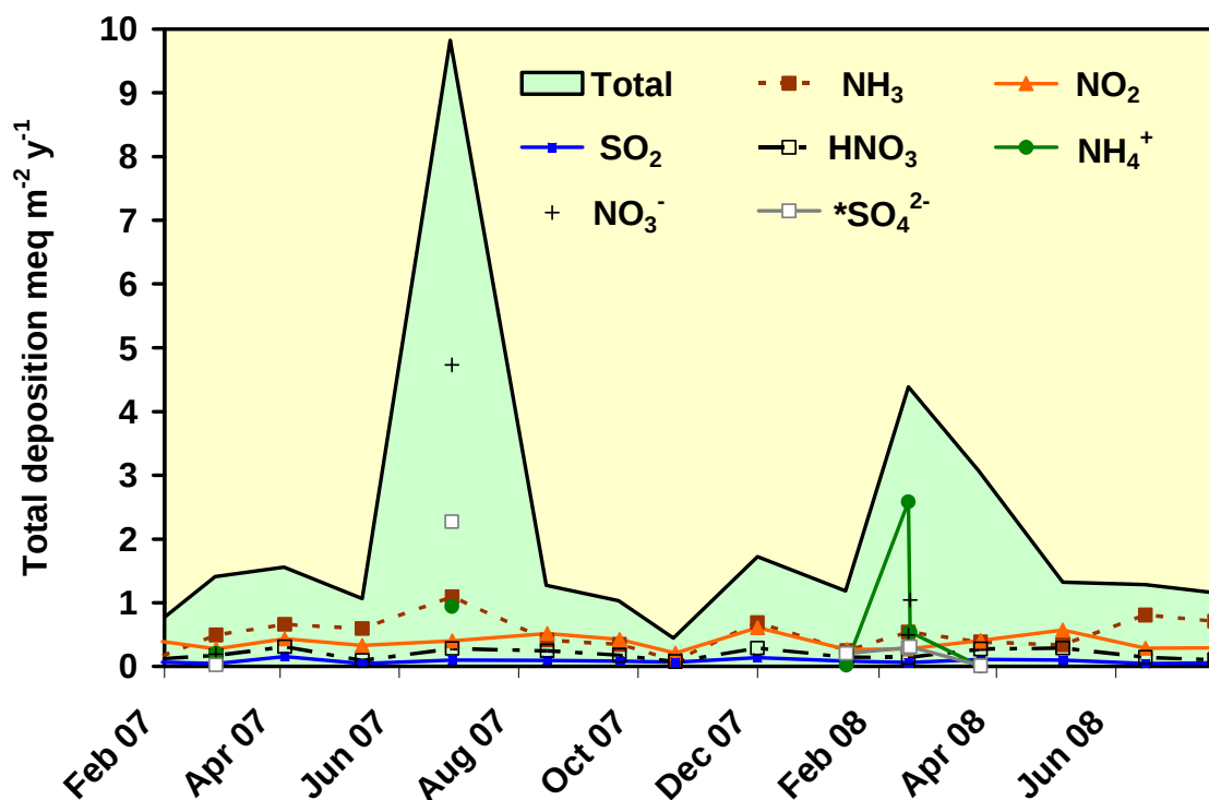
Figure 35. Total annual deposition of nitrogen and sulfur at site 8 during 2007/2008.
