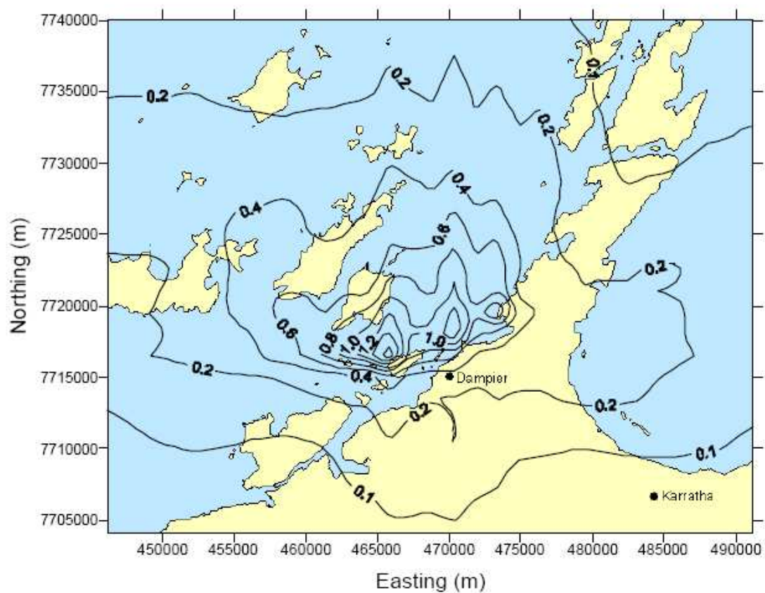
Figure 43. TAPM predicted annual sulfur dioxide deposition ( \text{kg ha}^{-1} \text{yr}^{-1} ) for existing industry (SKM, 2003).
