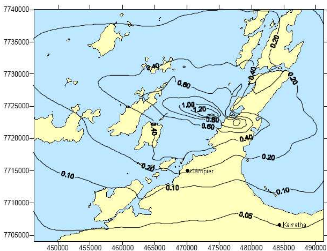
Figure 39. CALPUFF predicted annual nitrogen dioxide concentrations (ppb) for existing industry, (SKM, 2003).
