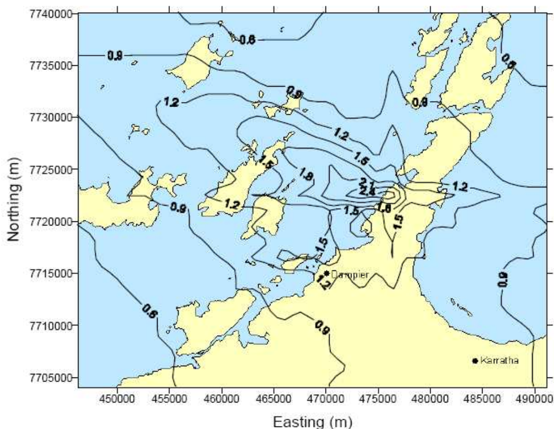
Figure 38. TAPM predicted annual nitrogen dioxide concentrations (ppb) for existing industry (SKM, 2003).
