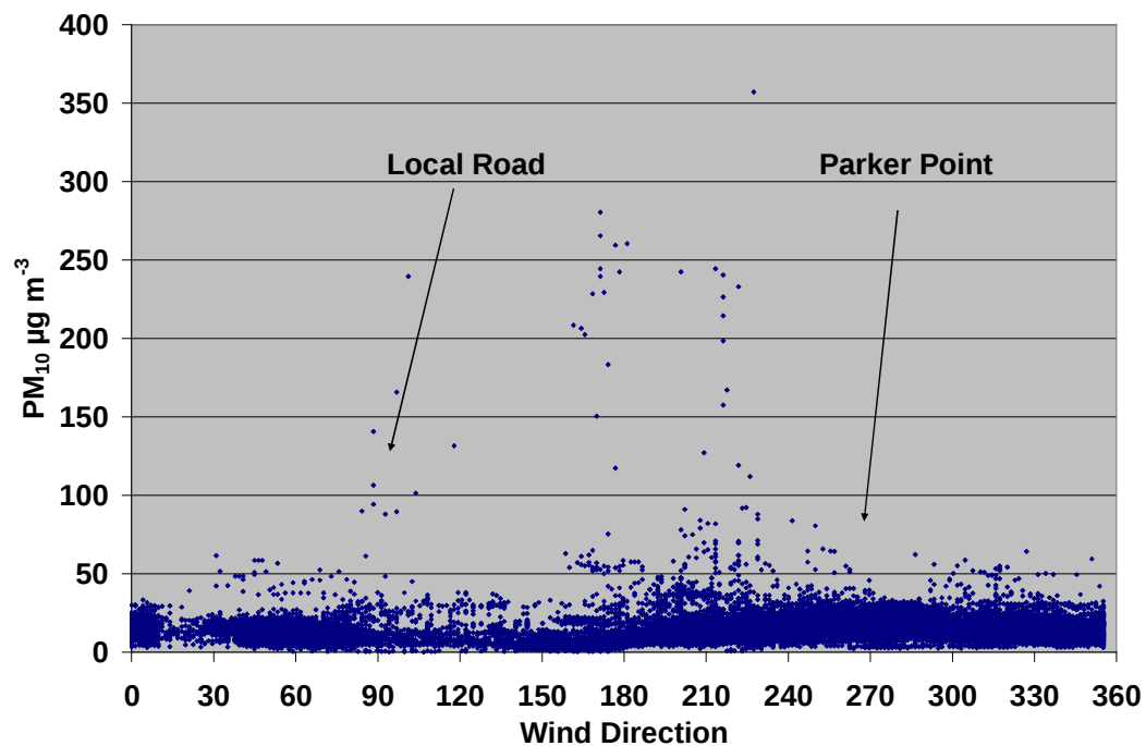
Figure 17. PM 10 concentration measured at Site 8 measured with DustTrak from 23 rd February 2005 until 23 rd March 2005, and plotted against wind direction measured at Site 8 at a frequency of two minutes. The average PM 10 concentration was 15.3 \mu\text{g m}^{-3} during that period.
