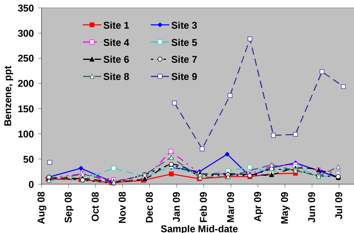
Figure 13c. Benzene concentrations at each site plotted against the sample mid-date for the 2008/2009 period.
