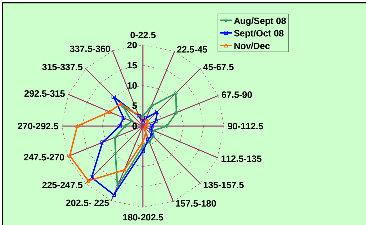
Figure 23. Wind roses recorded at site 8 for three periods from 13 th August 2008 – 22 nd September 2008, 22 nd September 2008 – 28 th October 2008 and 28 th October 2008 – 1 st December 2008.
