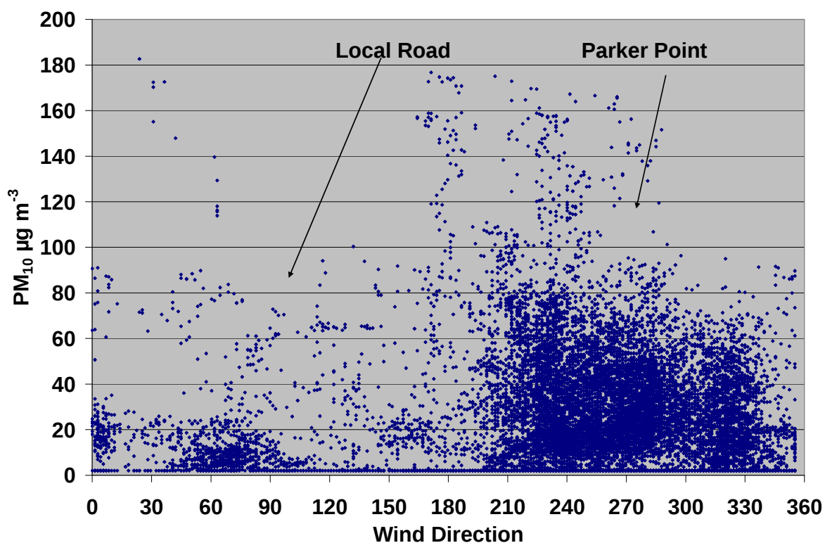
Figure 19. PM 10 concentrations plotted against wind direction at Site 8 from October 16th 2007 to November 8th 2007. The average PM 10 concentration for this period was 27.2 µg m -3 .
