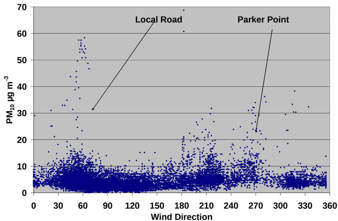
Figure 20. PM 10 concentrations plotted against wind direction at Site 8 from June 16th 2008 to July 14th 2008. The average PM 10 concentration for this period was 4.4 µg m -3 .
