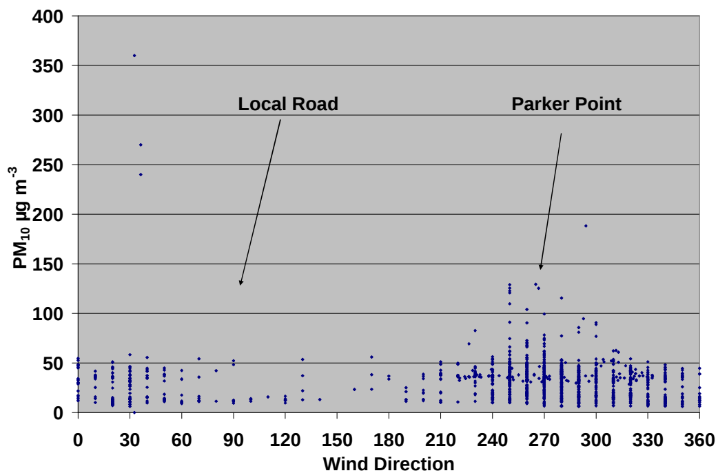
Figure 16. PM 10 concentration measured at Site 8 measured with DustTrak from 18 th January 2005 until 16 th February 2005, and plotted against wind direction measured at Karratha Airport at a frequency of thirty minutes. The average PM 10 concentration was 31.6 \mu\text{g m}^{-3} during that period.
