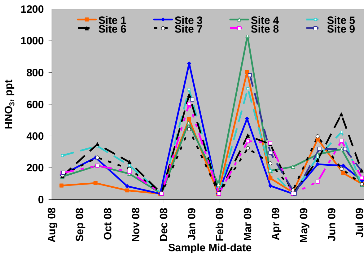
Figure 12c. Nitric acid concentrations plotted against the mid-date of the sampling period from August 2008 to August 2009.
