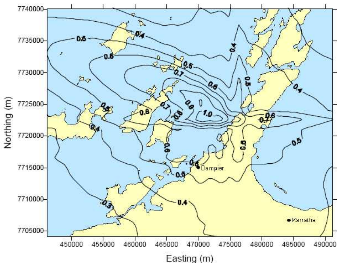
Figure 40. TAPM predicted annual nitrogen dioxide deposition ( \text{kg ha}^{-1} \text{yr}^{-1} ) for existing industry, (SKM, 2003).
