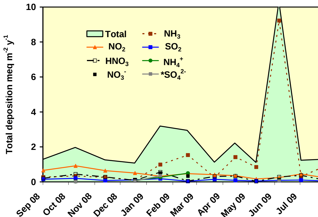
Figure 37. Total annual deposition of nitrogen and sulfur at site 6 during 2008/2009.
