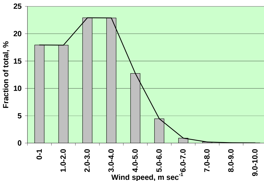
Figure 27. Frequency distribution of wind speeds at site 8 during the 2008/2009 sampling period.
