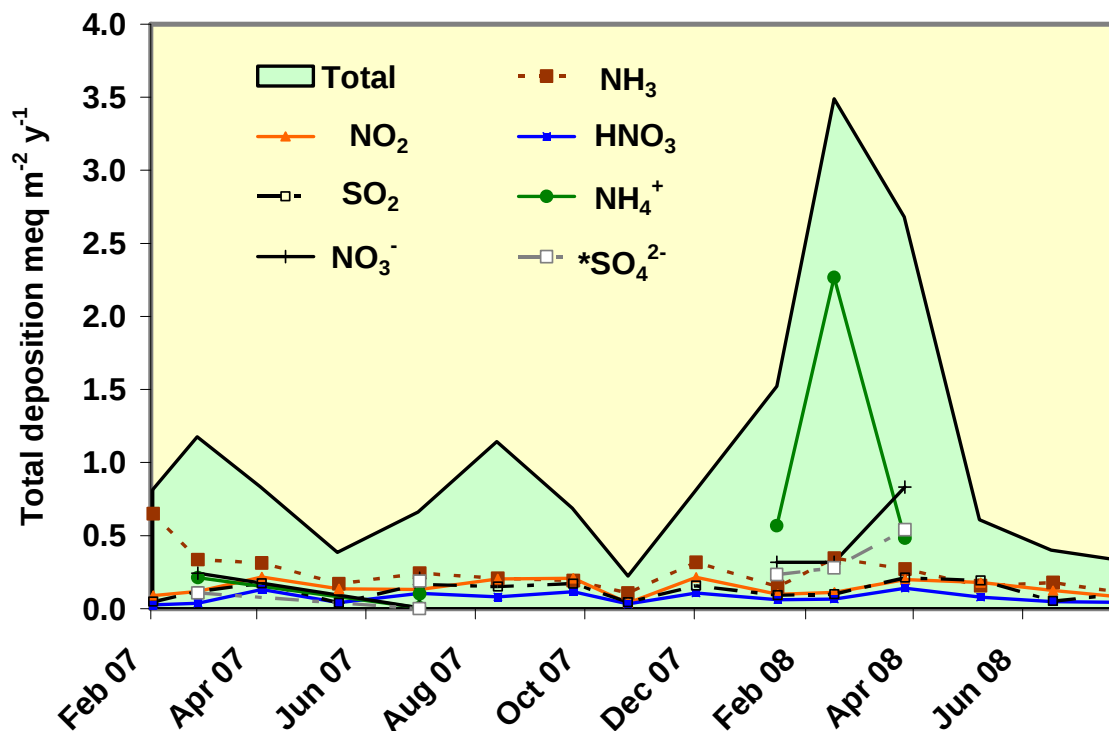
Figure 32. Total annual deposition of nitrogen and sulfur at site 3 during 2007/2008.
