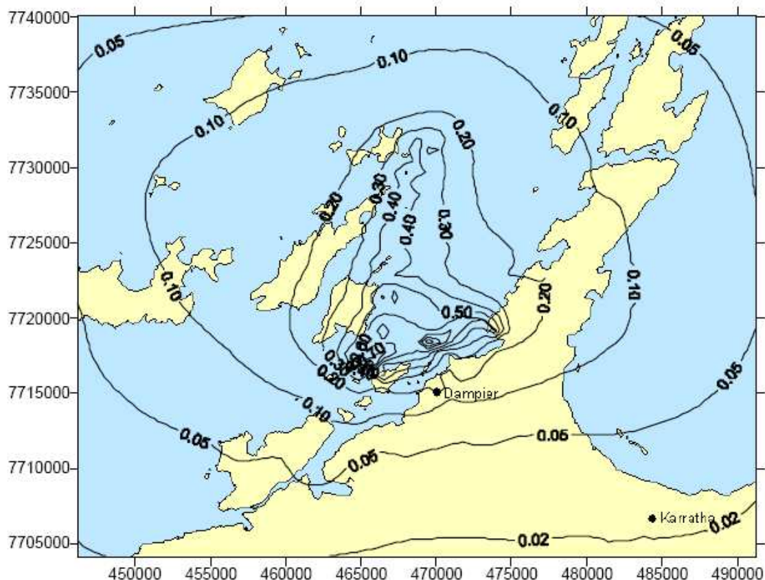
Figure 42. CALPUFF predicted annual sulfur dioxide concentrations (ppb) for existing industry (SKM, 2003).
