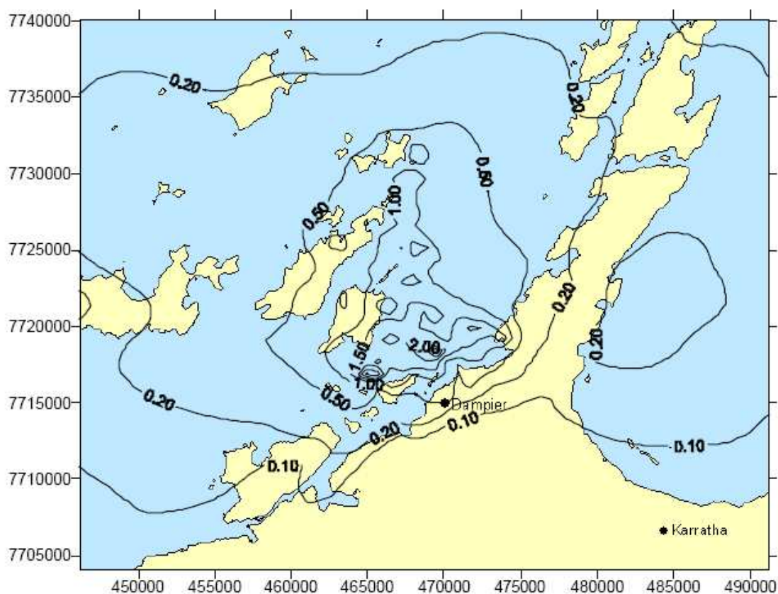
Figure 44. CALPUFF predicted annual sulfur dioxide deposition ( \text{kg ha}^{-1} \text{yr}^{-1} ) for existing industry (SKM, 2003).
