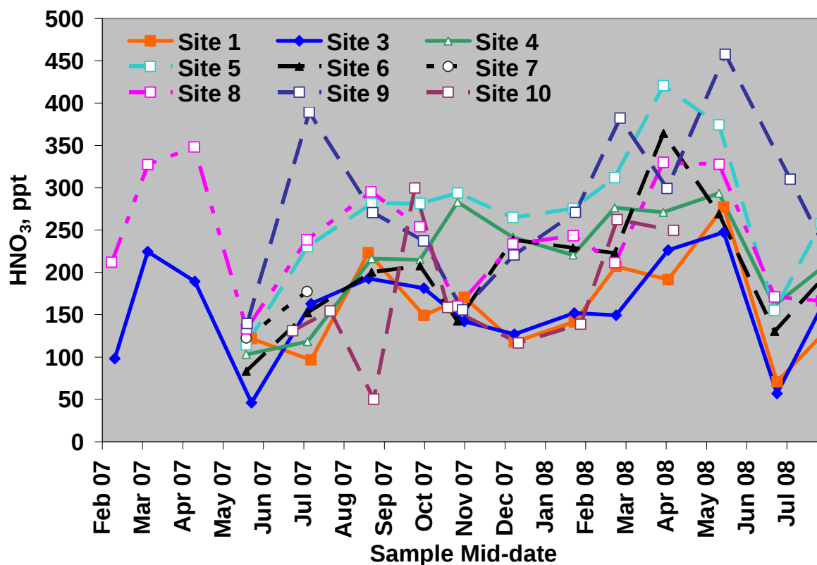
Figure 12b. Nitric acid concentrations plotted against the mid-date of the sampling period from February 2007 to August 2008.
