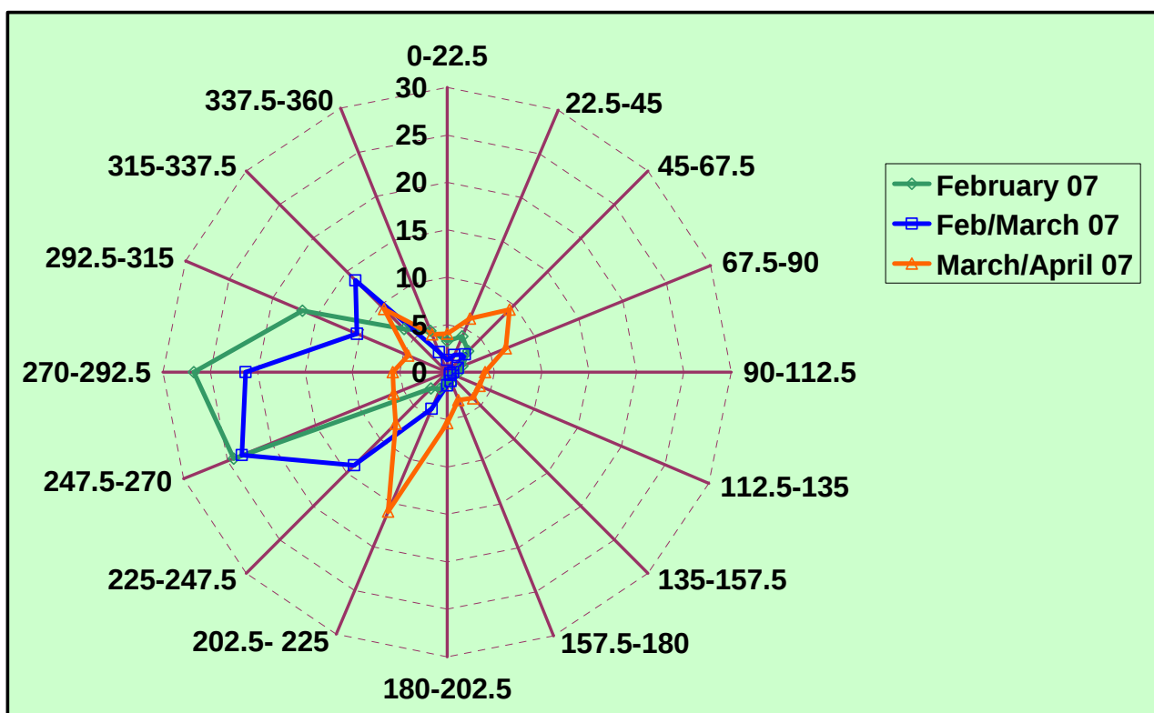
Figure J5. Wind roses recorded at site 8 for three periods from 24 th January 2007 – 22 nd February 2007, February 2007 – 20 th March 2007 and 20 th March 2007 – 3 rd May 2007.
