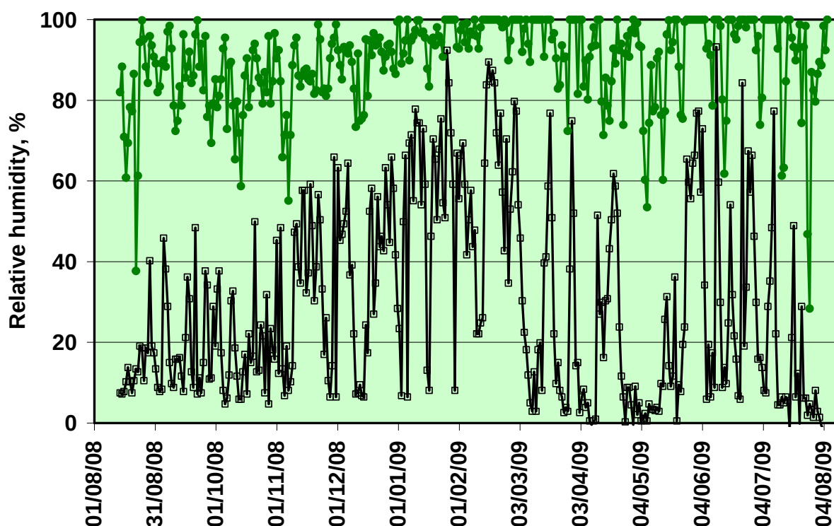
Figure 29. Daily maximum and minimum relative humidity measurements at site 8 during the 2008/2009 sampling period.
