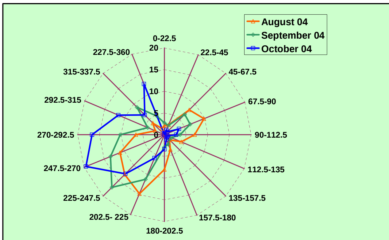
Figure J1. Wind roses recorded at site 8 from August 2004 to October 2004.
