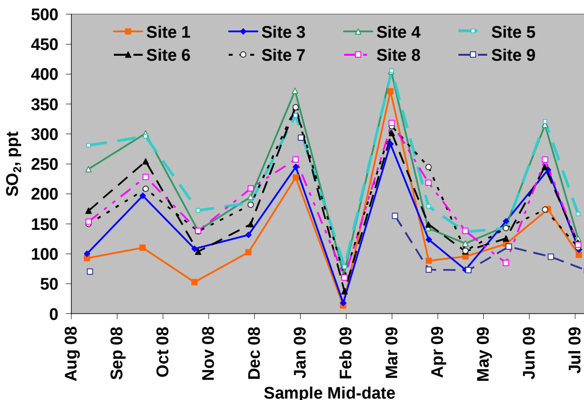
Figure 11c. Sulfur dioxide concentrations plotted against the mid-date of the sampling period from August 2008 to August 2009.
