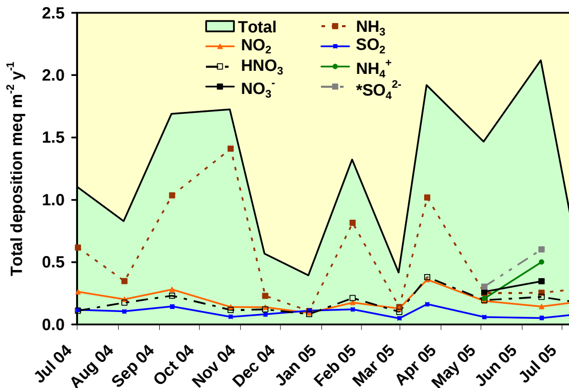
Figure 31. Total annual deposition of nitrogen and sulfur at site 3 during 2004/2005.
