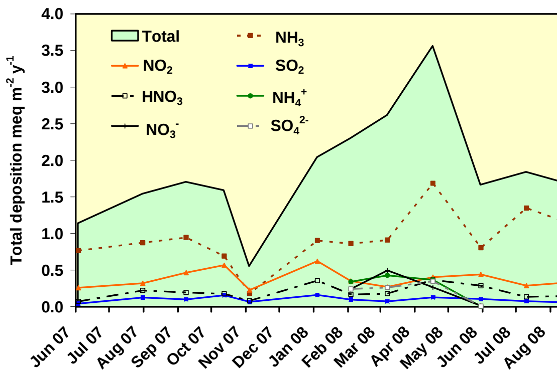
Figure 34. Total annual deposition of nitrogen and sulfur at site 6 during 2007/2008.
