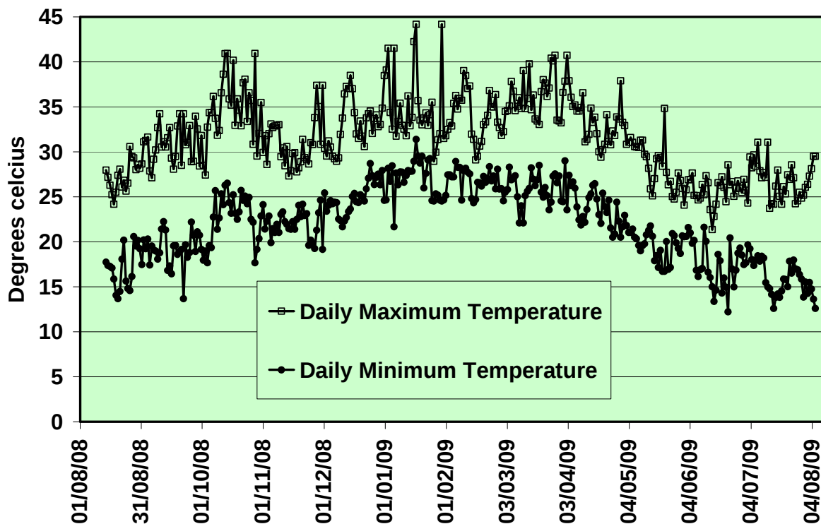
Figure 28. Daily maximum and minimum temperatures at site 8 during the 2008/2009 sampling period.
