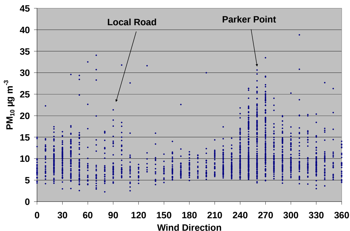
Figure 18. PM 10 concentration measured at Site 8 measured with DustTrak from 23 rd March 2005 until 28 th April 2005, and plotted against wind direction measured at Karratha Airport at a frequency of thirty minutes. The average PM 10 concentration was 10.4 µg m -3 during that period.
