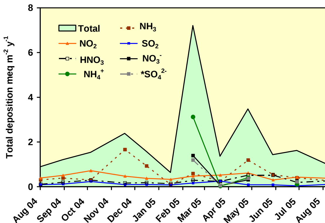
Figure 33. Total annual deposition of nitrogen and sulfur at site 6 during 2004/2005.
