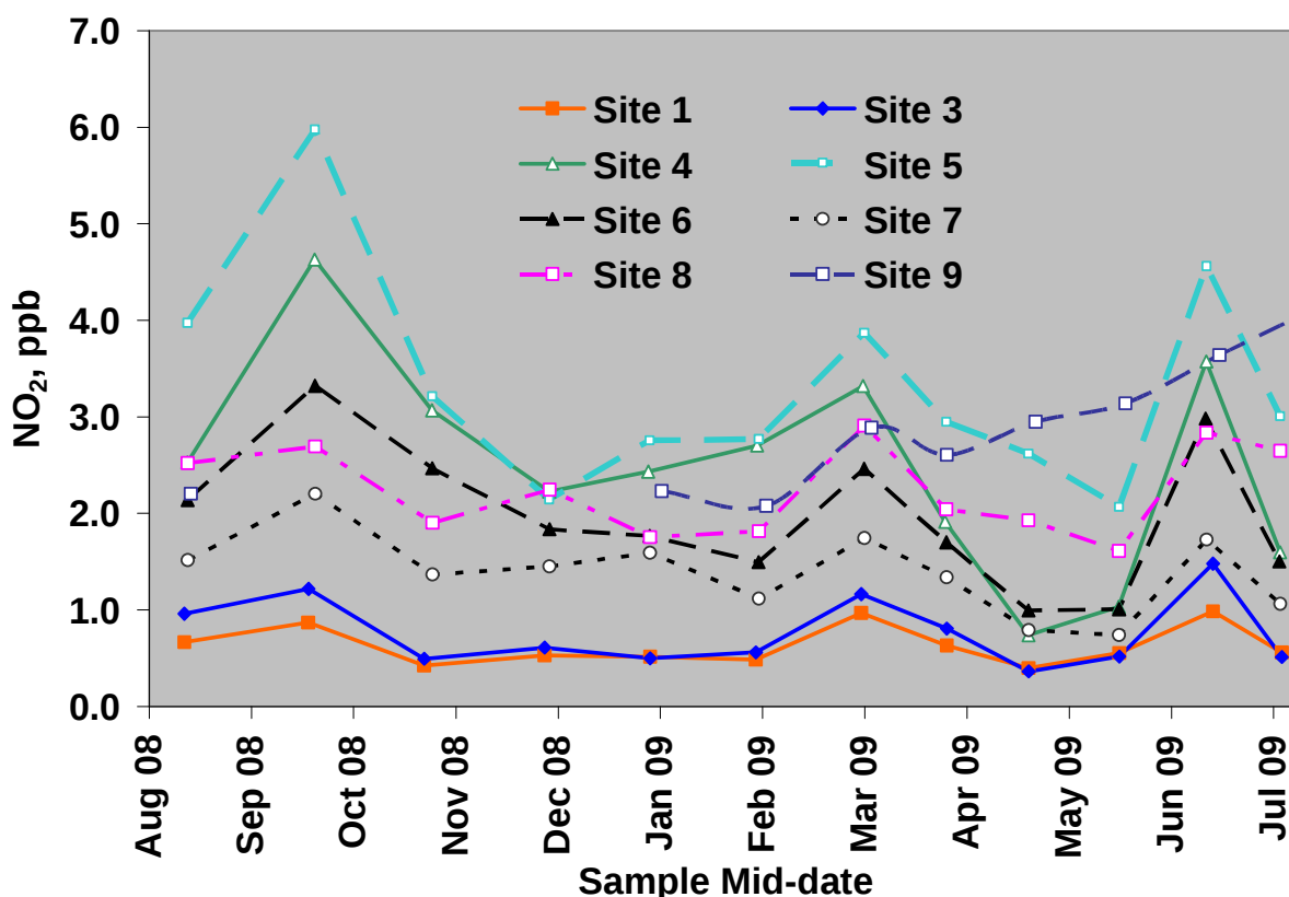
Figure 10c. Nitrogen dioxide concentrations plotted against the mid-date of the sampling period from August 2008 to August 2009.
