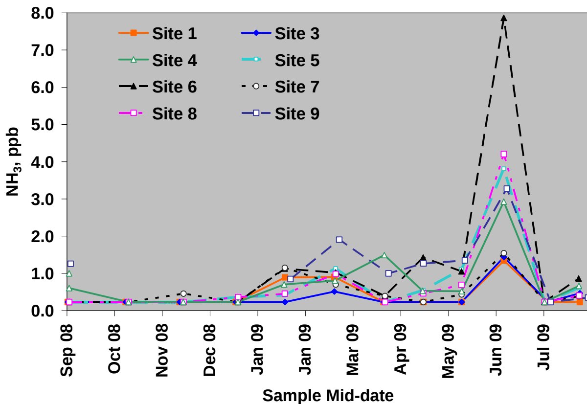
Figure 9c. Ammonia concentrations plotted against the mid-date of the sampling period from August 2008 to August 2009.
