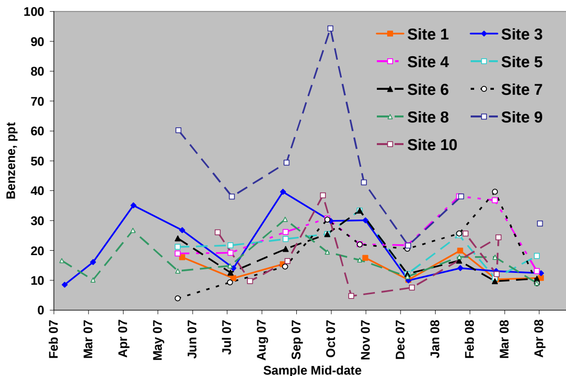
Figure 13b. Benzene concentrations at each site plotted against the sample mid-date for the 2007/2008 period.
