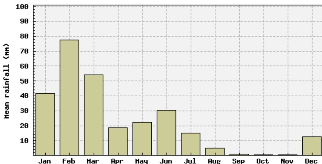
Figure 30. Rainfall distribution at Karratha Airport from 1972 to 2009 ( http://reg.bom.gov.au/jsp/ncc/cdio/cvg/av?p_stn_num=004083&p_prim_element_index=18&p_display_type=statGraph&period_of_avg=ALL&normals_years=allYearOfData&staticPage= ).
