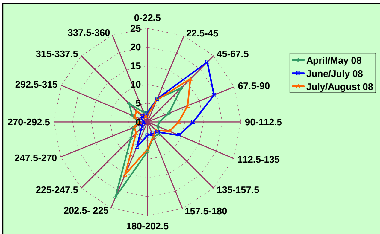
Figure J8. Wind roses recorded at site 8 for three periods from 21 st April 2008 – 3 rd June 2008, 3 rd June 2008– 14 th July 2008 and 14 th July 2008 – 13 th August 2008.
