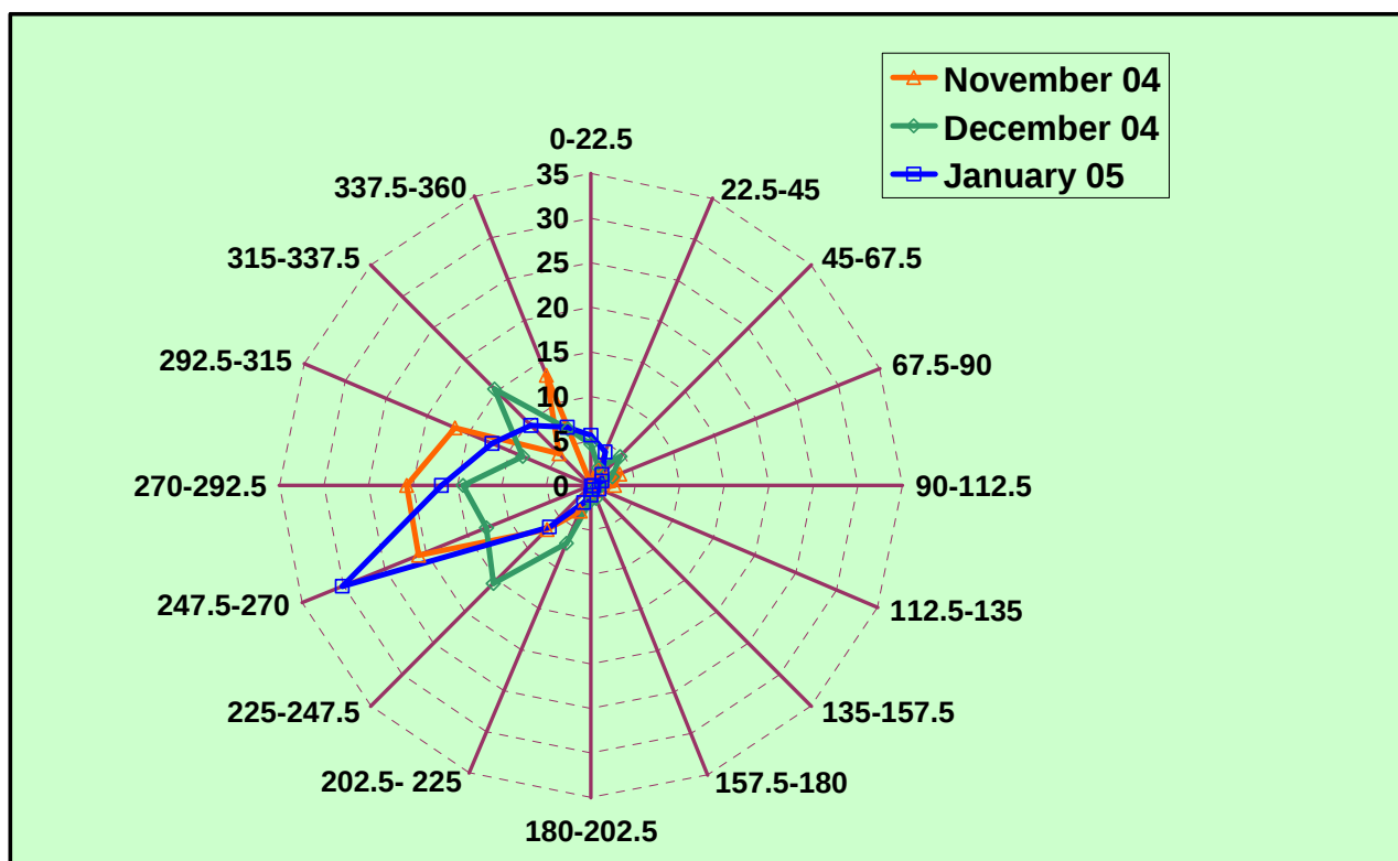
Figure J2. Wind roses recorded at site 8 from November 2004 to January 2005.
