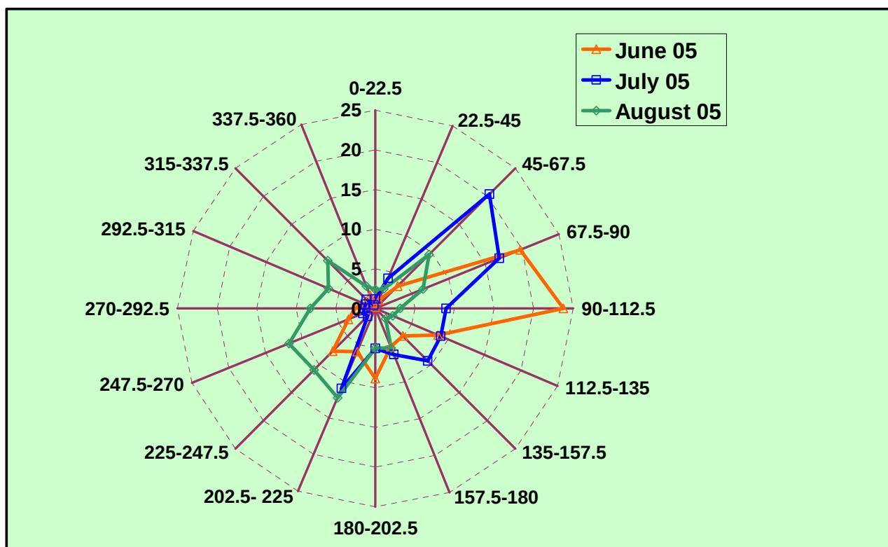
Figure J4. Wind roses recorded at site 8 from June 2005 to August 2005
