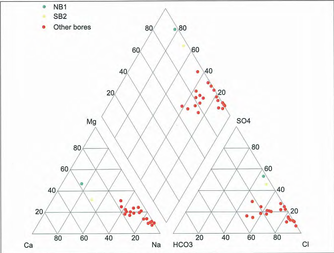
Figure 4. Piper trilinear diagram of selected chemical analyses of groundwaters.
