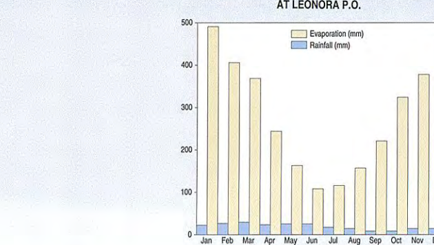
MEAN MONTHLY RAINFALL AND EVAPORATION AT LEONORA P.O.
