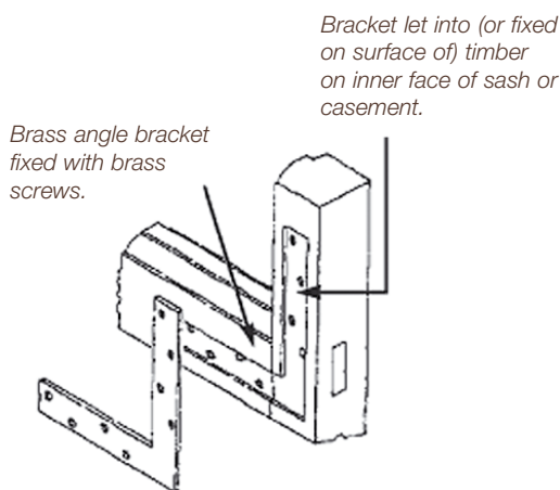
Diagram from A. Townsend & M. Martyn, The Repair of Wood Windows , SPAB, London
