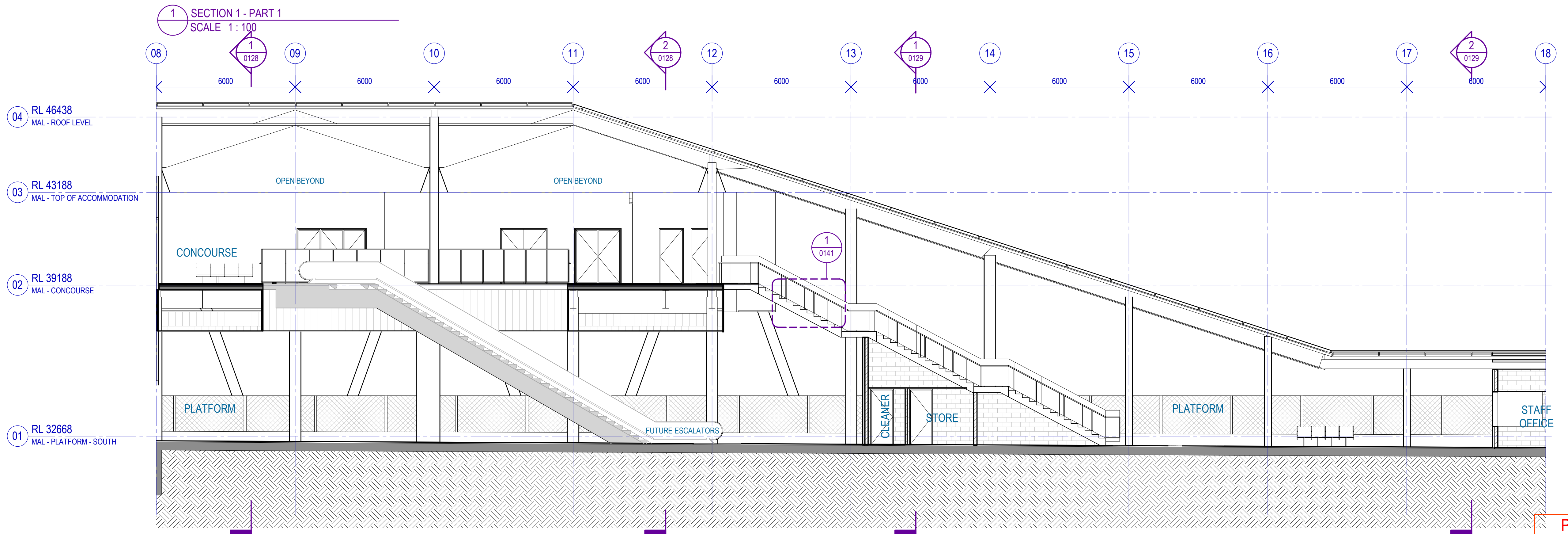
2 SECTION 1 - PART 2 SCALE 1 : 100
