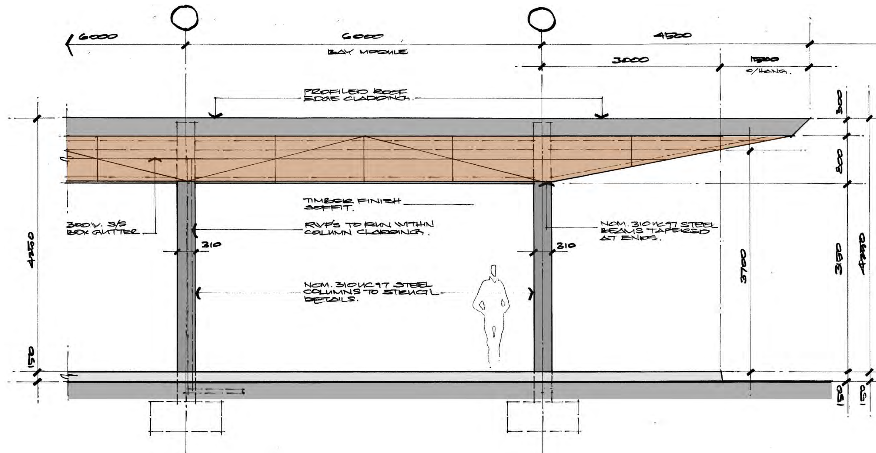
1 BUS CANOPY - ASYMETRICAL - FRONT ELEVATION SCALE 1 : 40
