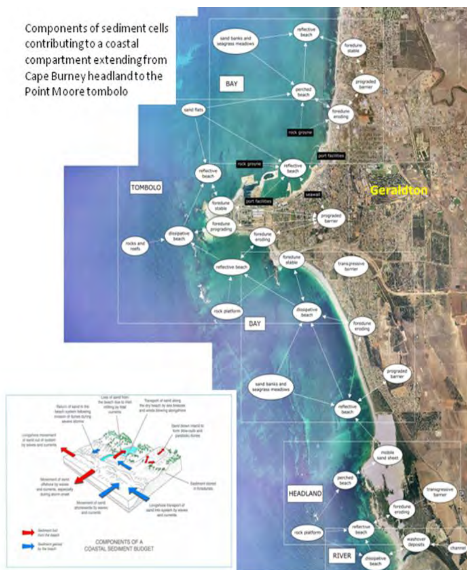
Figure 2-2: Sediment Budget Components
