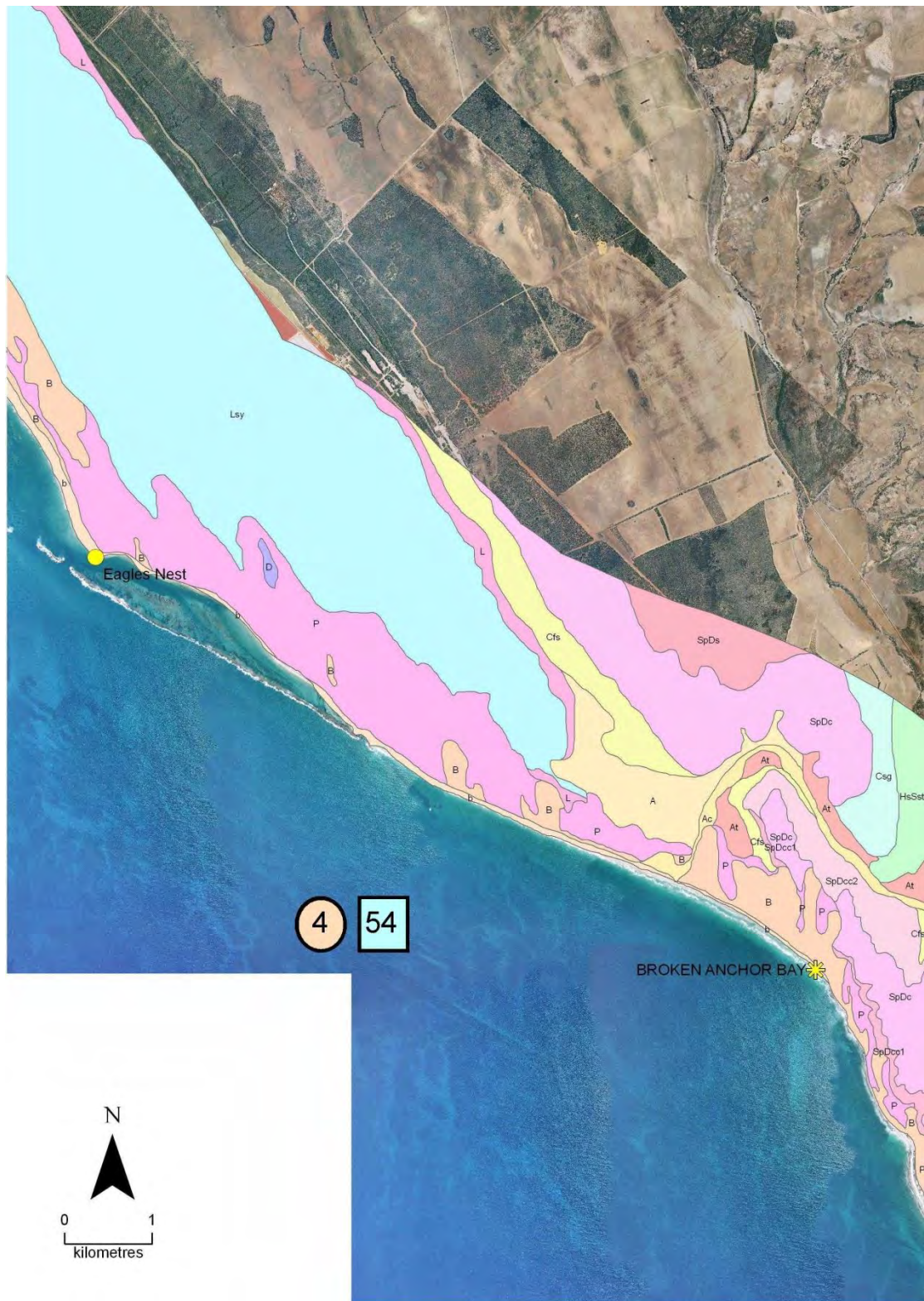
Figure C - 15: Landforms for Cell 54
