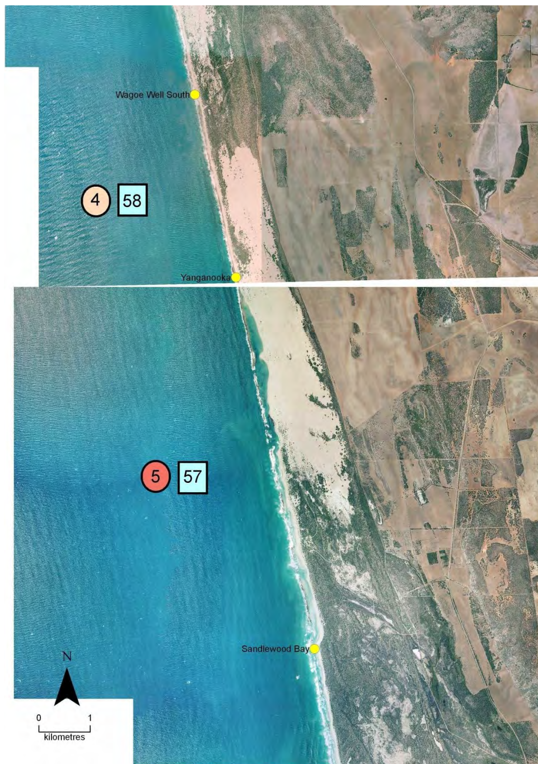
Figure C - 10: Vulnerability for Cells 57-58
