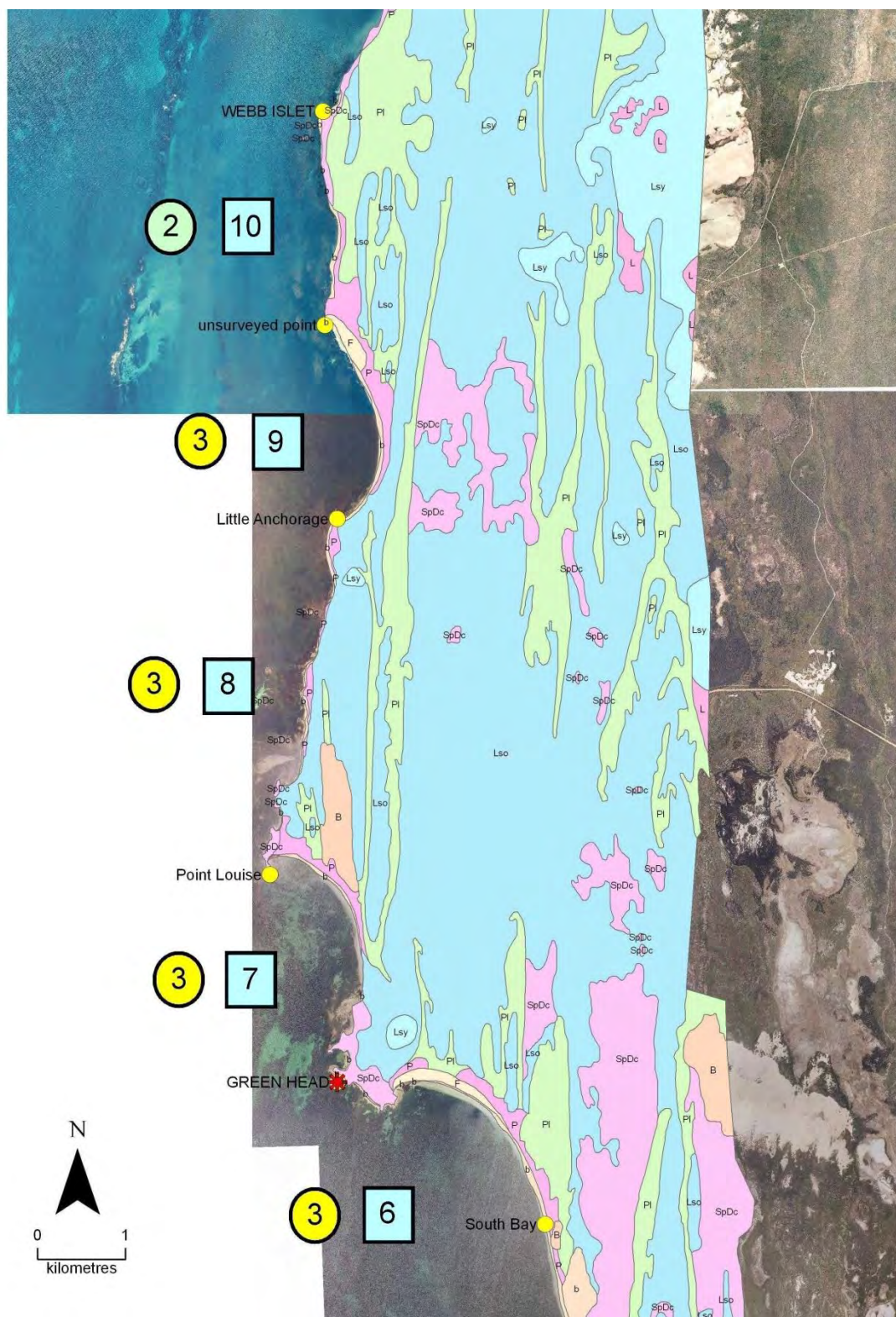
Figure C - 53: Landforms for Cells 6-10
