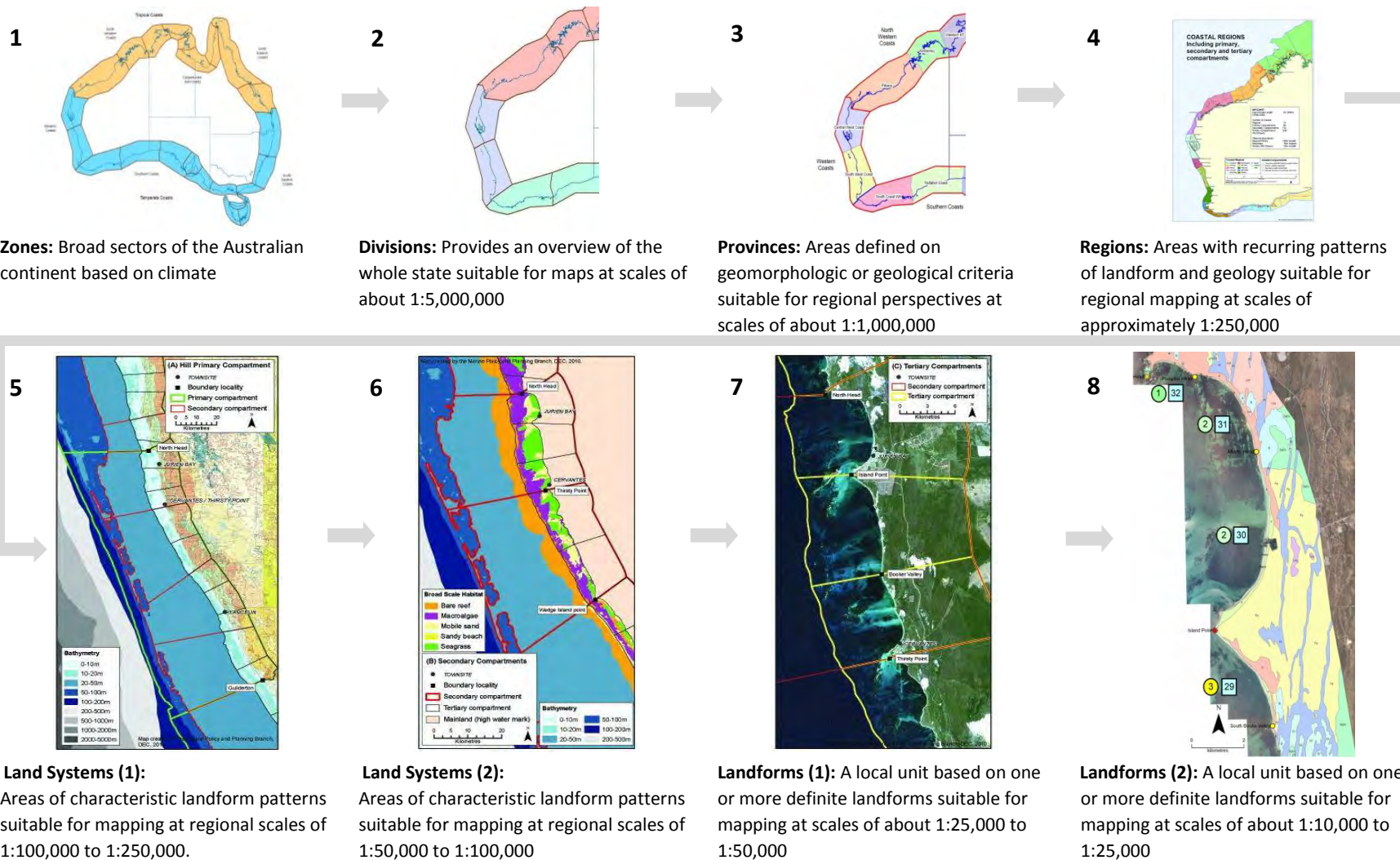
Figure 3-1: Coastal Land Systems Hierarchy
