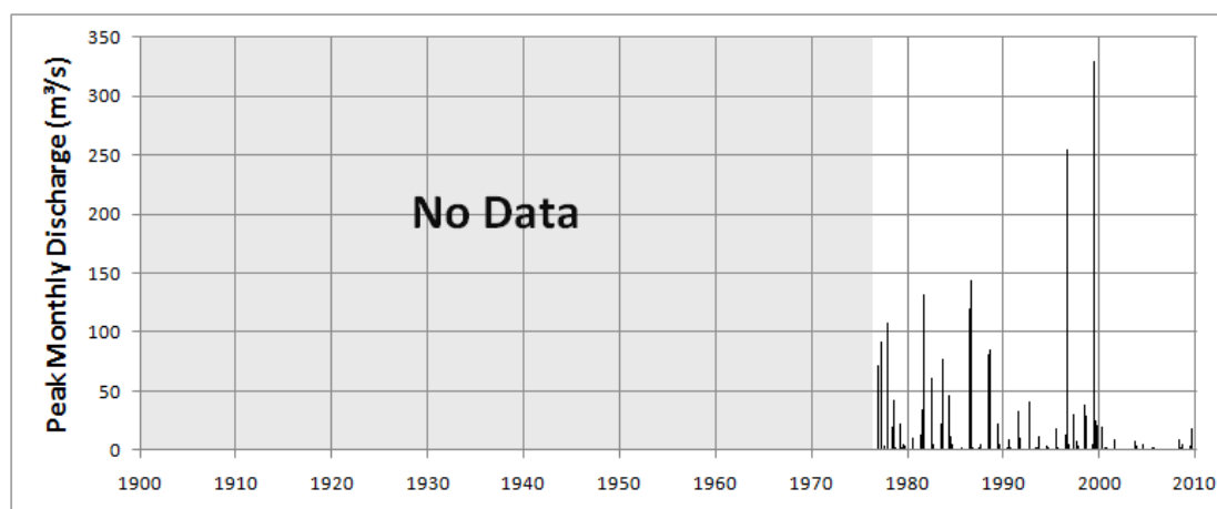
Figure 4-27: Peak Monthly Discharge at Utakarra approximately 10 km upstream of the Chapman River mouth (Source: Department of Water)
