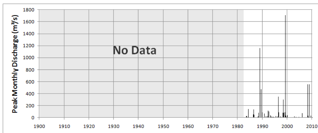
Figure 4-24: Peak Monthly Discharge at Mountain Bridge approximately 18 km upstream of the Irwin River mouth (Source: Department of Water)
