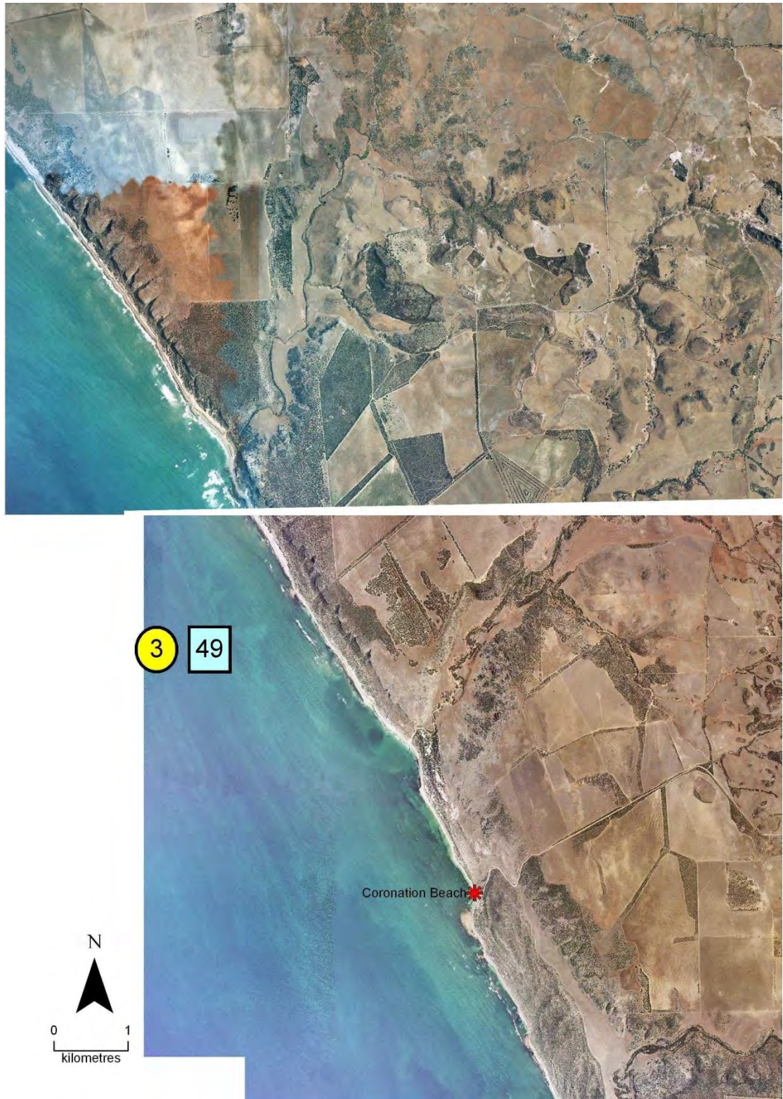
Figure C - 22: Vulnerability for Cell 49
