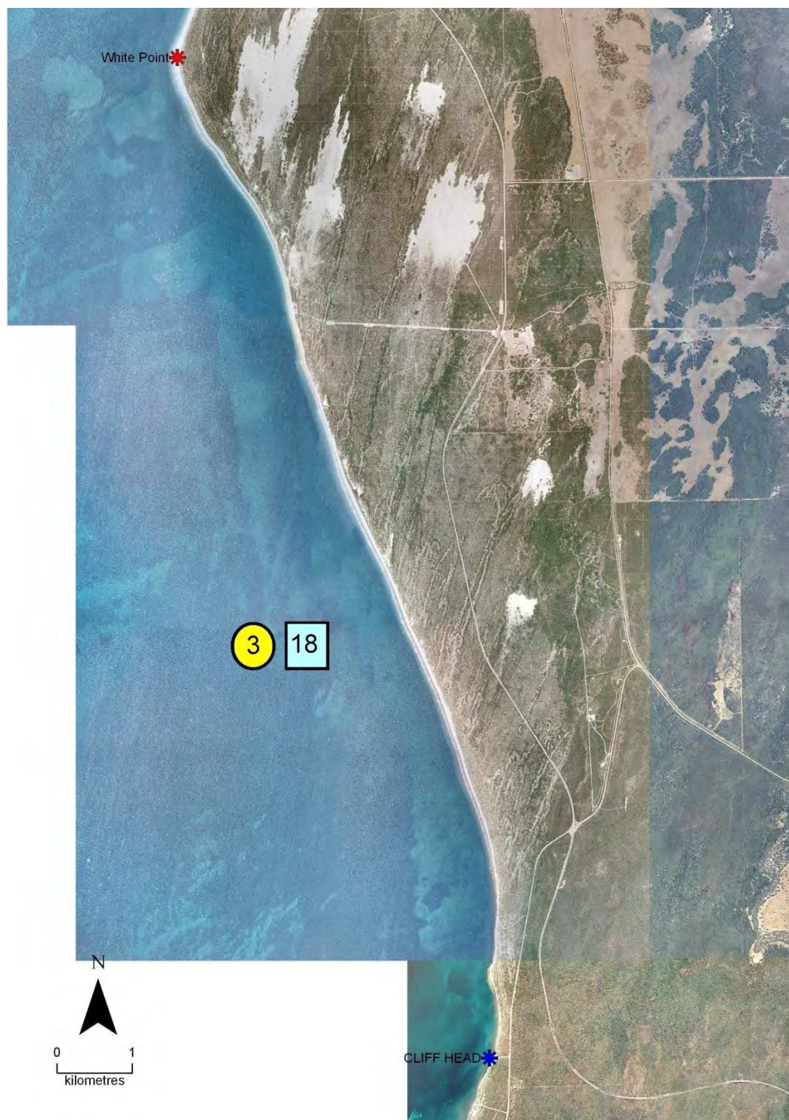
Figure C - 40: Vulnerability for Cell 18
