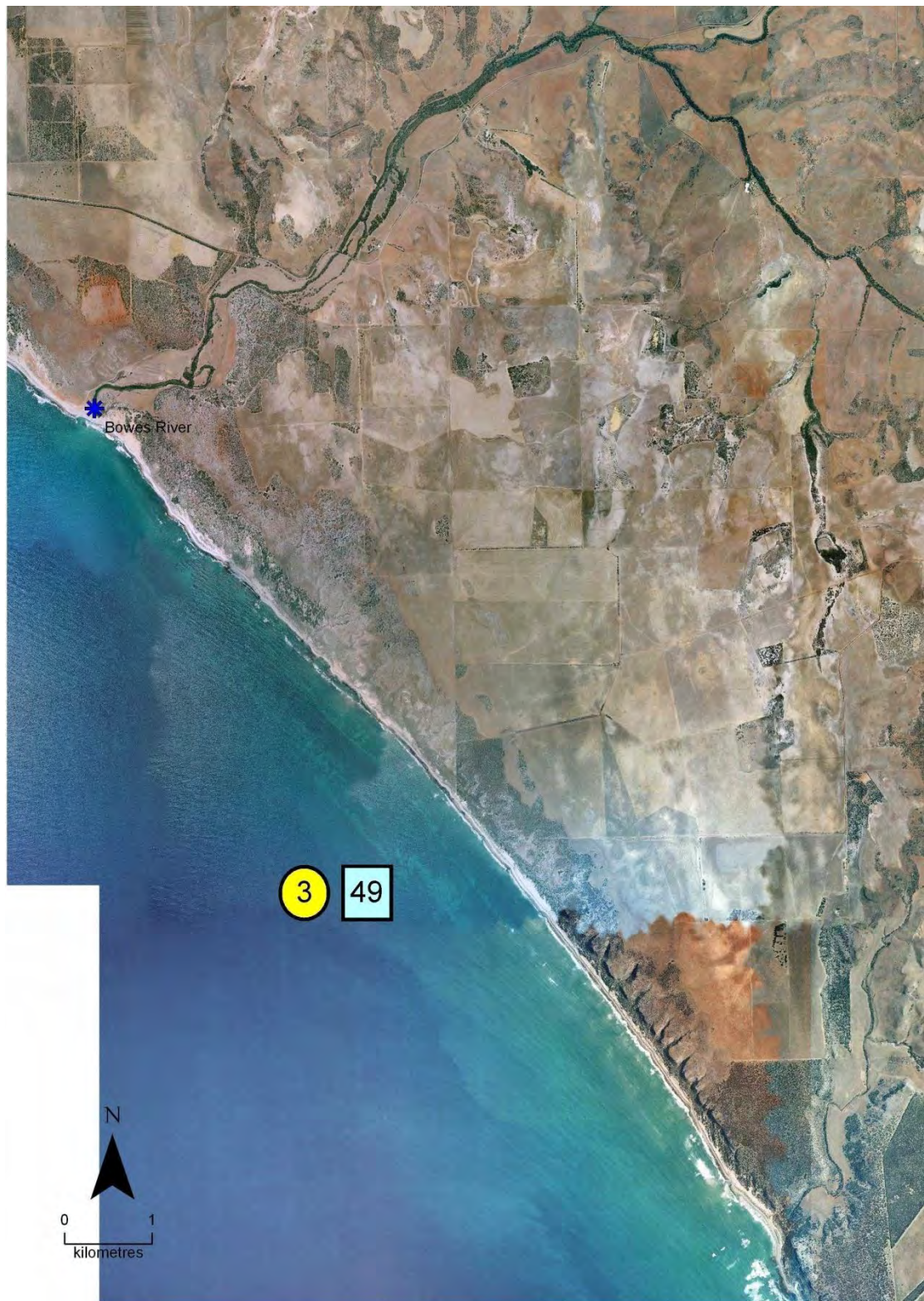
Figure C - 20: Vulnerability for Cell 49
