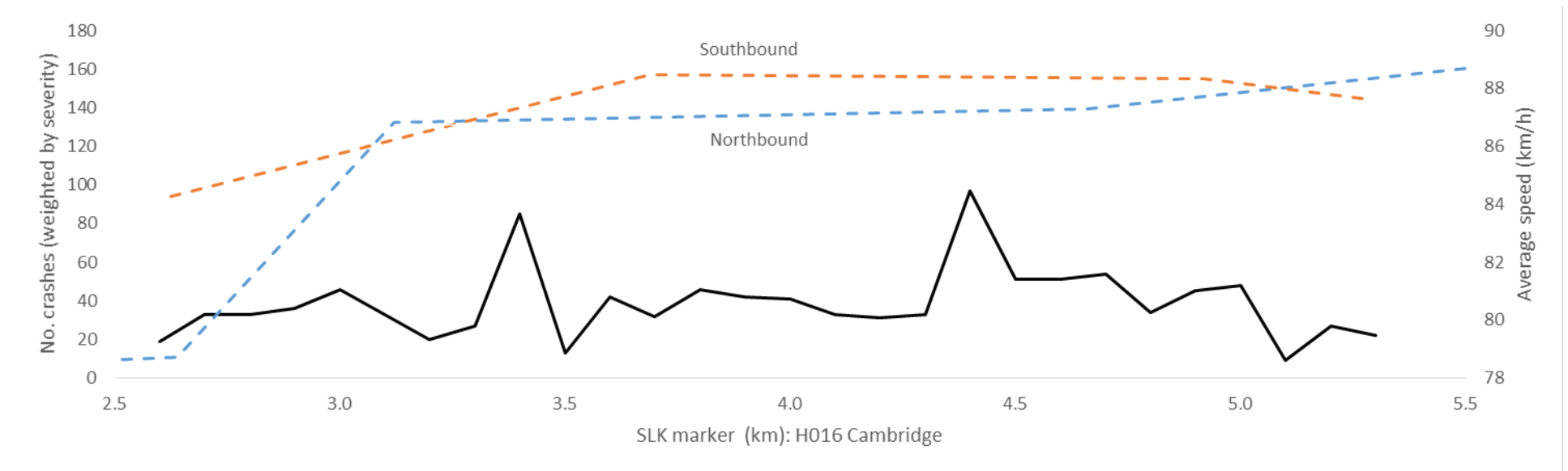
Figure 18 Distribution of sum of weighted crashes (interval 0.1km) and motor-vehicle speed, H016 Cambridge
