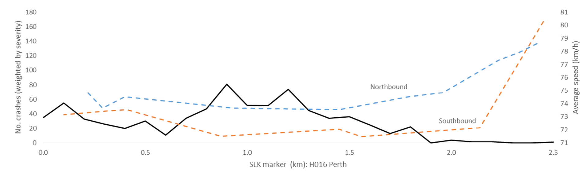
Figure 17 Distribution of sum of weighted crashes (interval 0.1km) and motor-vehicle speed, H016 Perth
