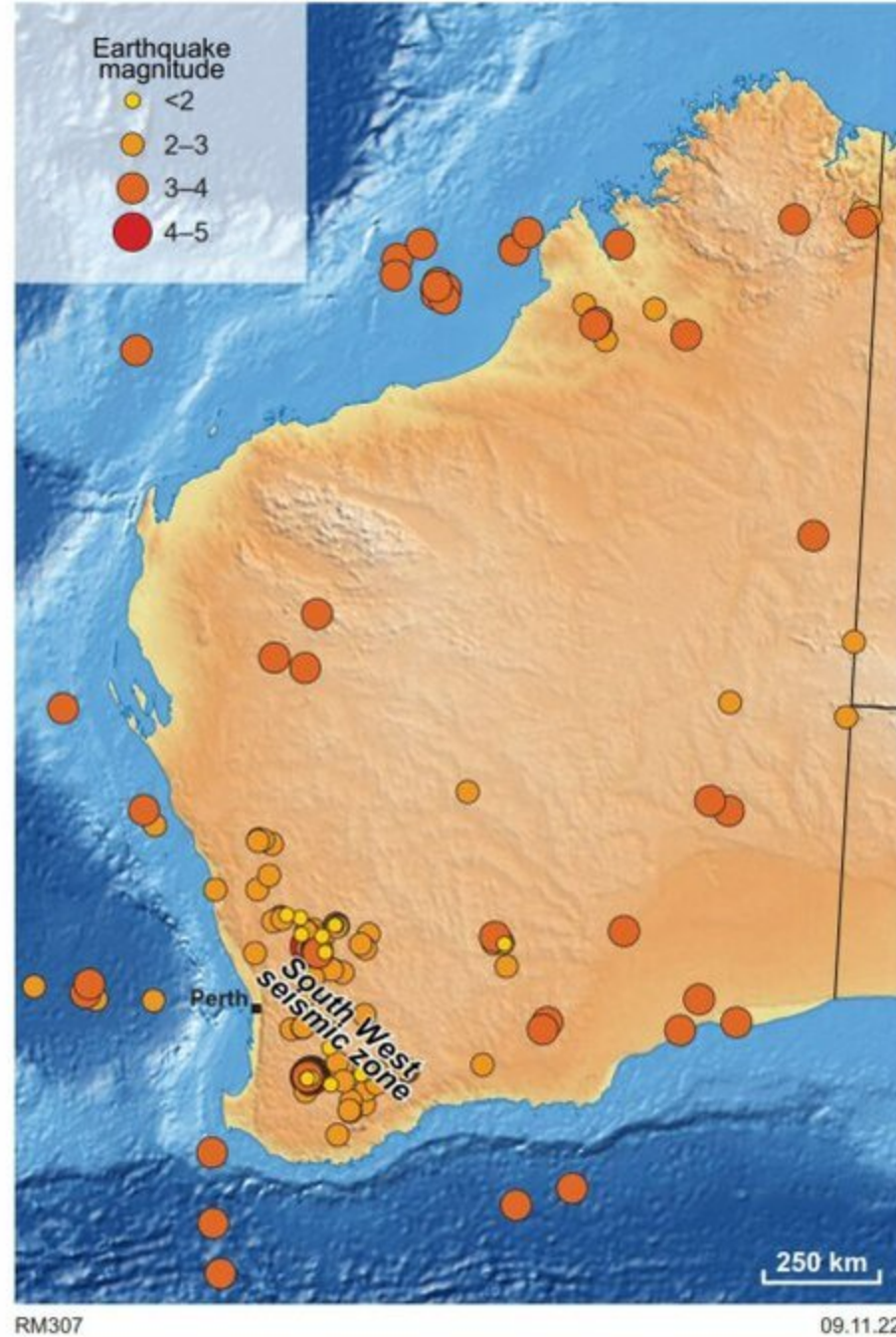
Earthquakes in Western Australia during 2022 as recorded by the Australian National Seismograph Network
